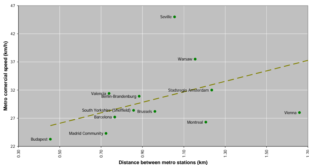
Graph 30. Link between metro stations separation and commercial speed
